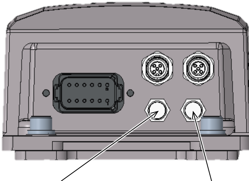
Main antenna connection part (GNSS1)
