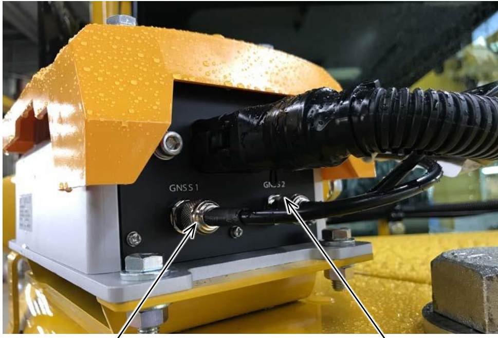
Main antenna connection part (GNSS1)
